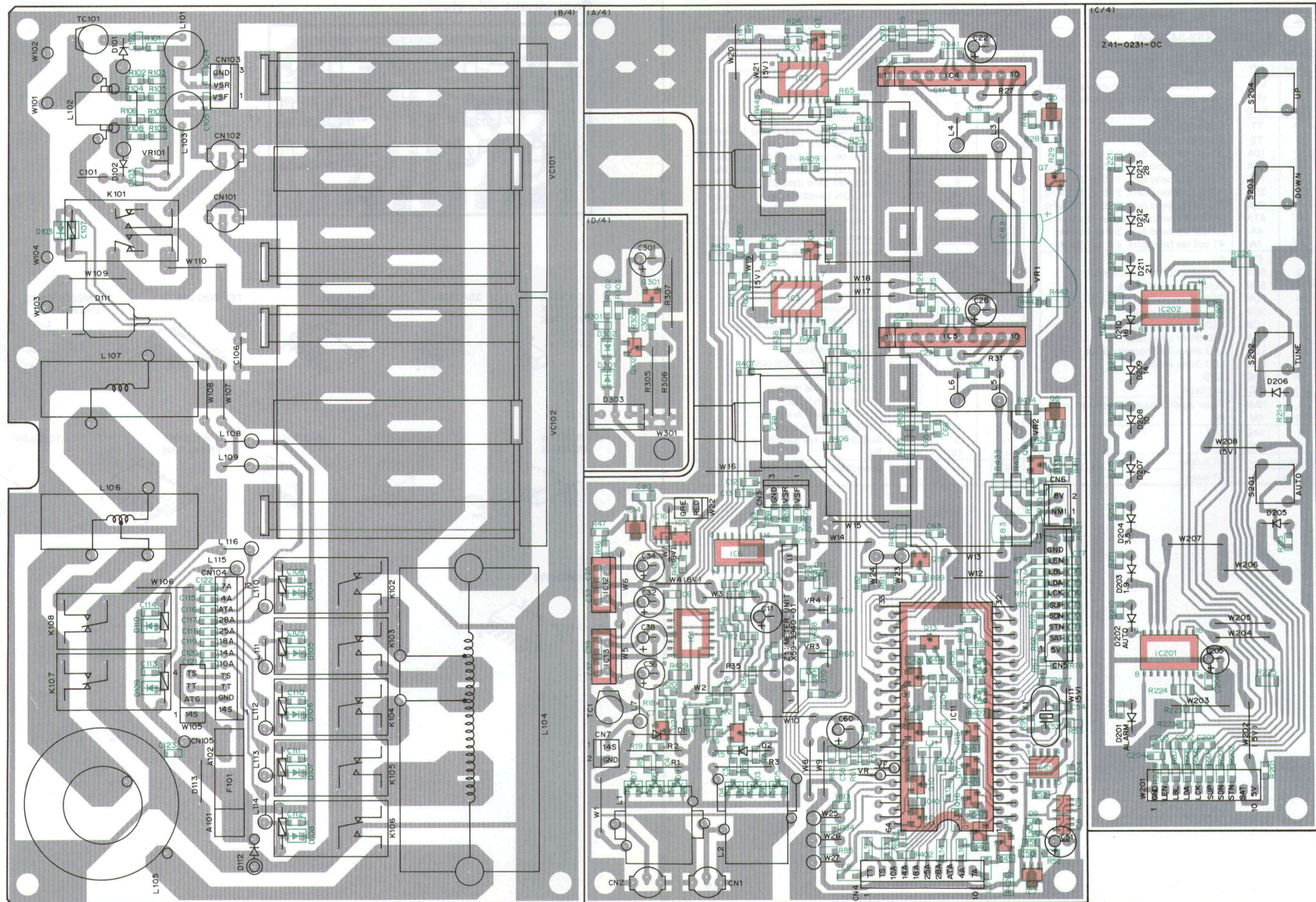
AT UNIT (X53-3470-00) Component side view
